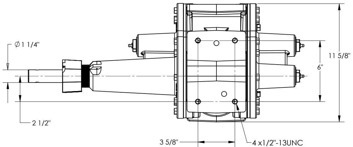
BOTTOM VIEW
