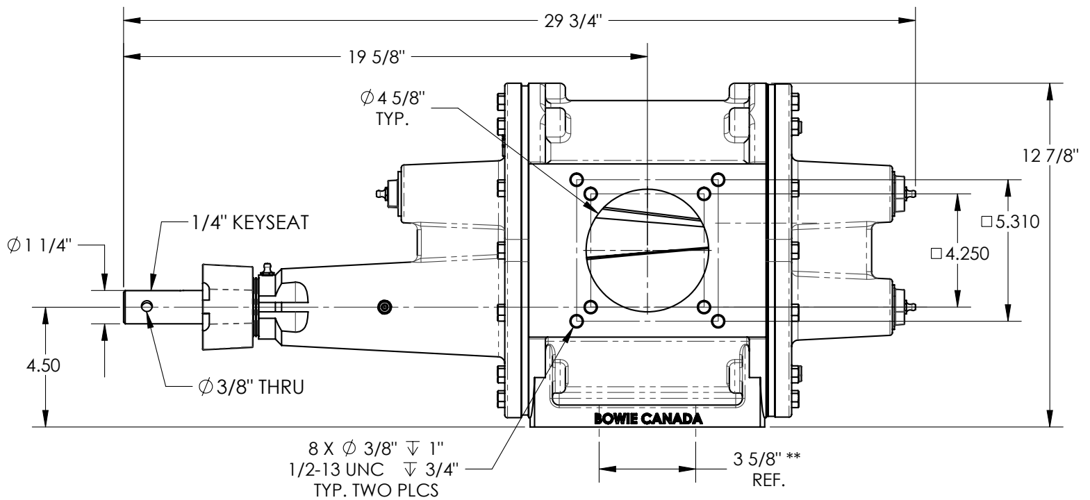
BOTTOM VIEW
